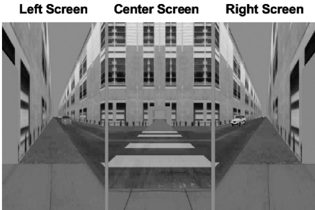
Figure 1. A sample still capture of the virtual reality street crossing task. Each image is representative of the wall in the CAVE on which it was presented. Although the street appears to be U shaped in the still image captures, when presented in the virtual viewing environment, the street appeared to run straight and seamlessly.
